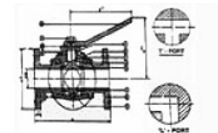
6. Válvula de bola 3Way Full Body Bore L ou T porto wp upto 100 bar
